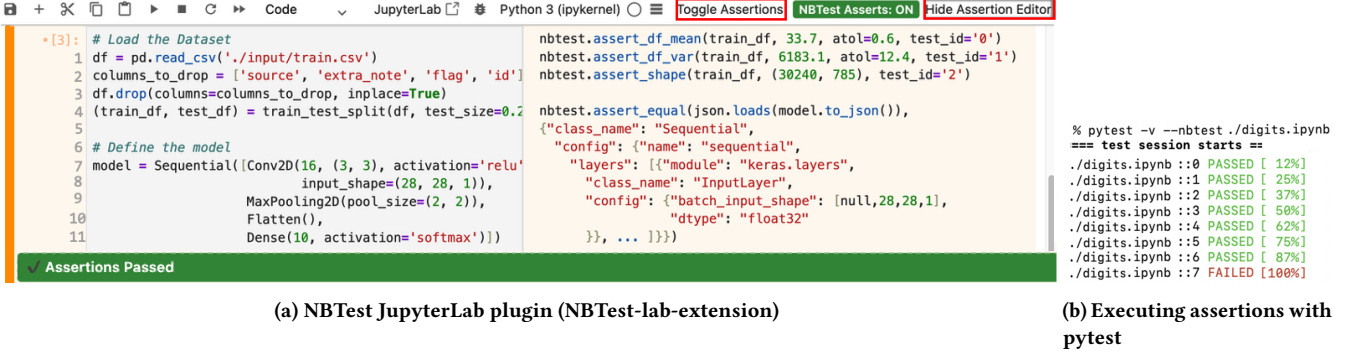
Figure 1: Example usage of NBTest. (a) shows NBTestGen assertions in a JupyterLab side panel, which can be hidden by Hide Assertion Editor button, or enabled/disabled with the Toggle Assertions button. The green message bar ( Assertions Passed ) indicates assertions passed. (b) shows pytest output for NBTest assertions.
